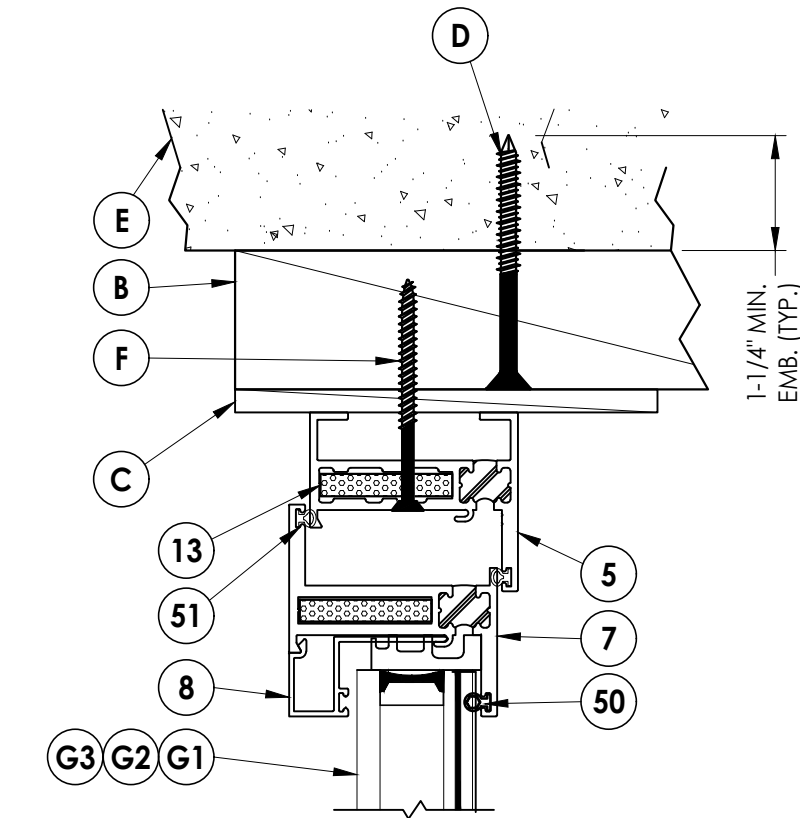
5 HORIZONTAL CROSS SECTION 4 Shown w/ 2X Buck Construction
