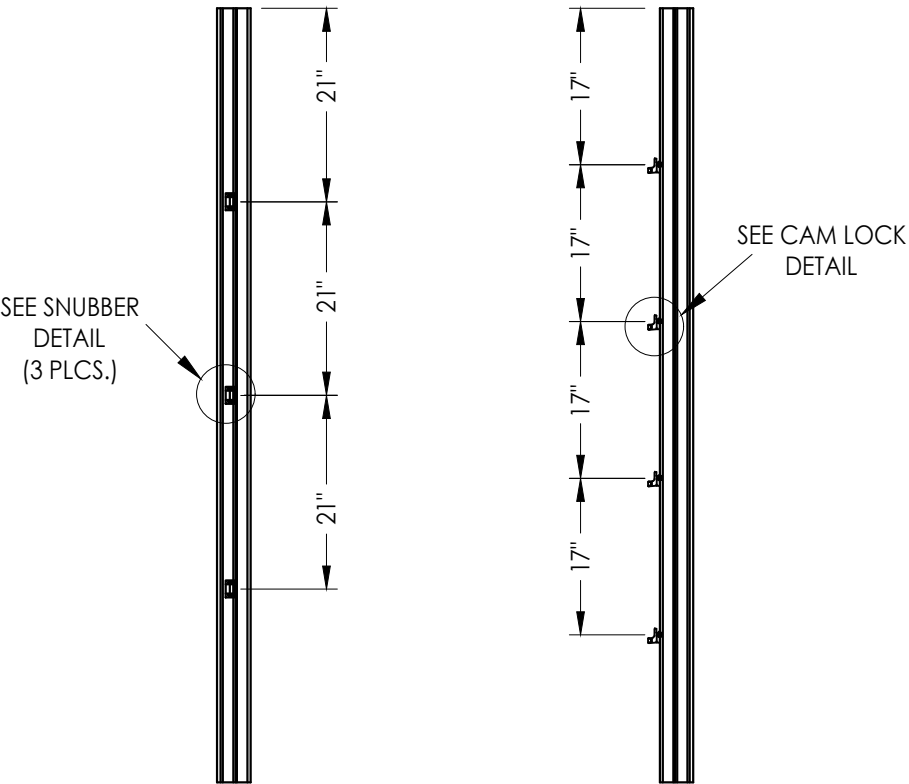
SNUBBERS JAMB
