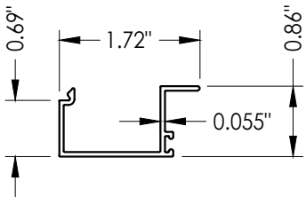
10 GLASS STOP 9/16"
